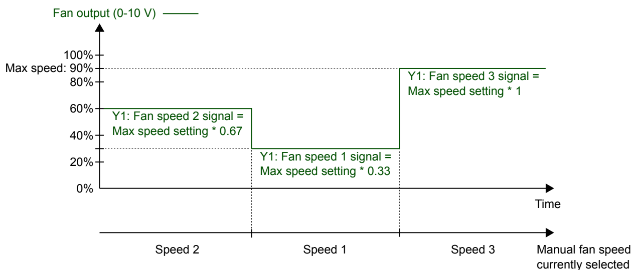
Figure 3-34 EC fan control behaviour in manual mode (fan speed 1, 2, or 3).
