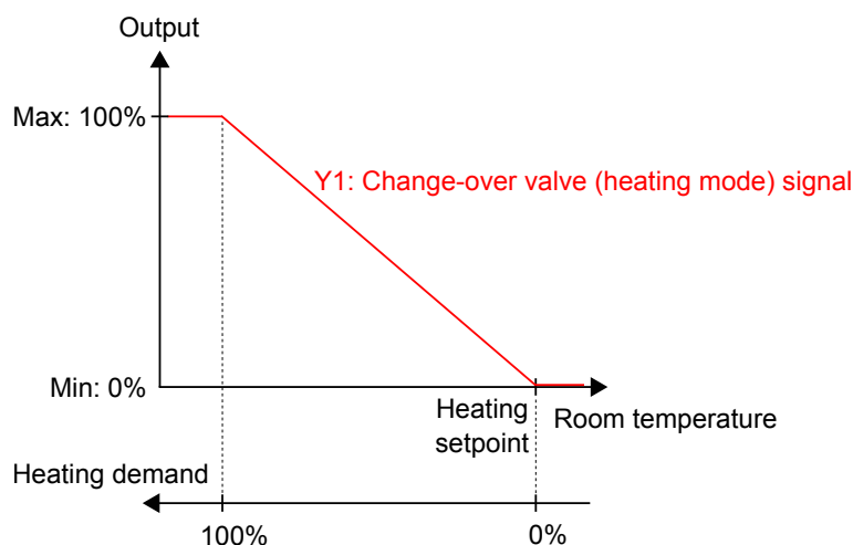
Figure 3-7 Control behaviour for the Heating/Cooling (change-over) controller mode when the controller is in heating mode.
