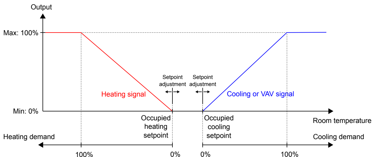
Figure 3-28 Control behaviour for the occupied and bypass controller state.
