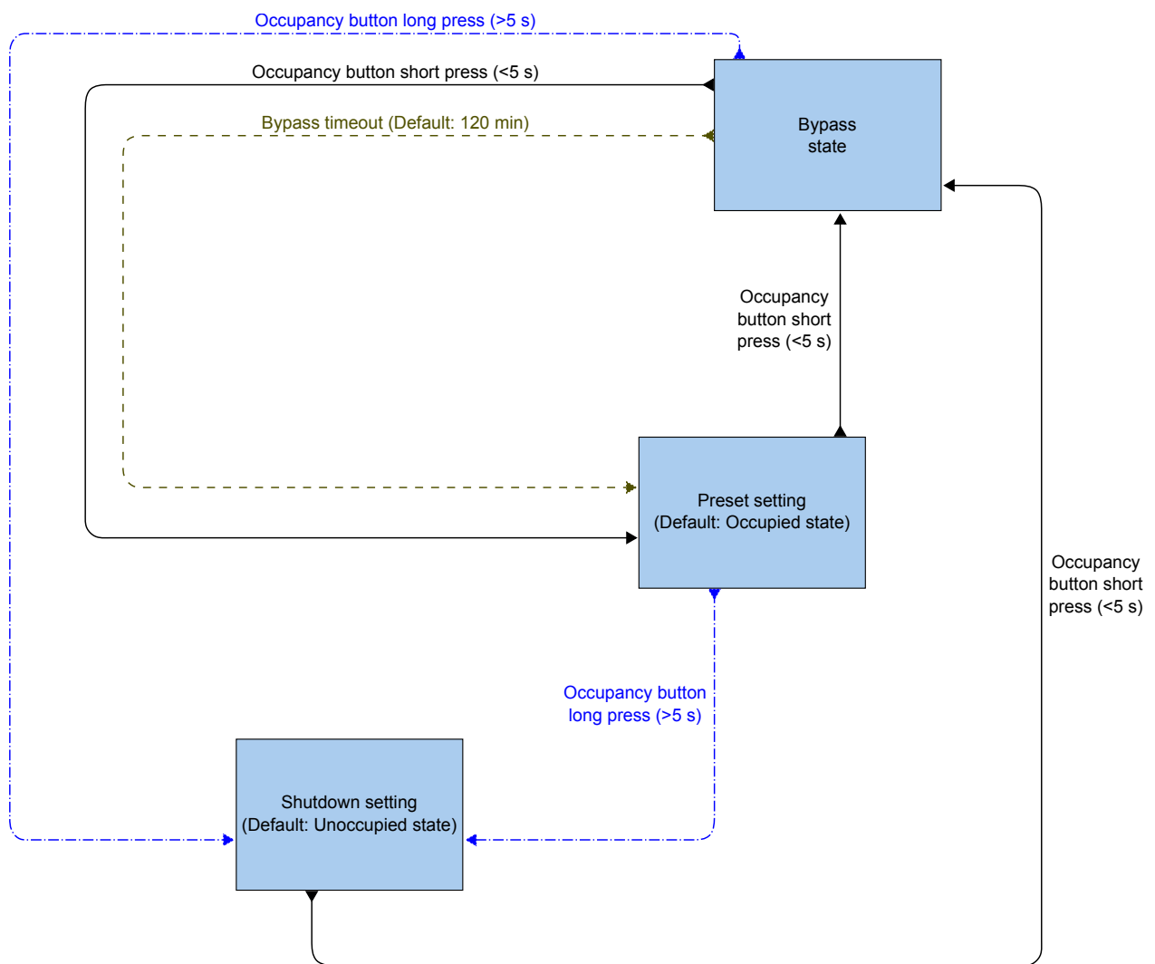
Figure 3-29 Flow chart describing controller state changes for when the occupancy (on/off) button on the room unit is used.
