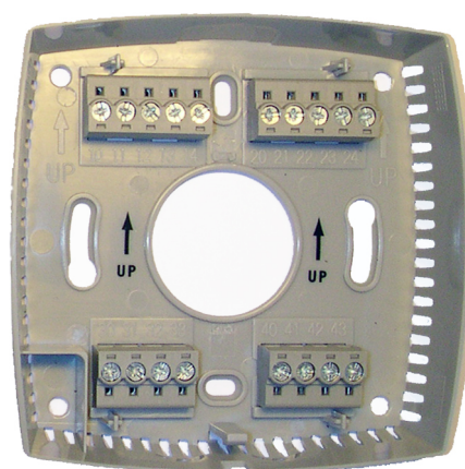
Current terminal type (1.1 mm pins).
