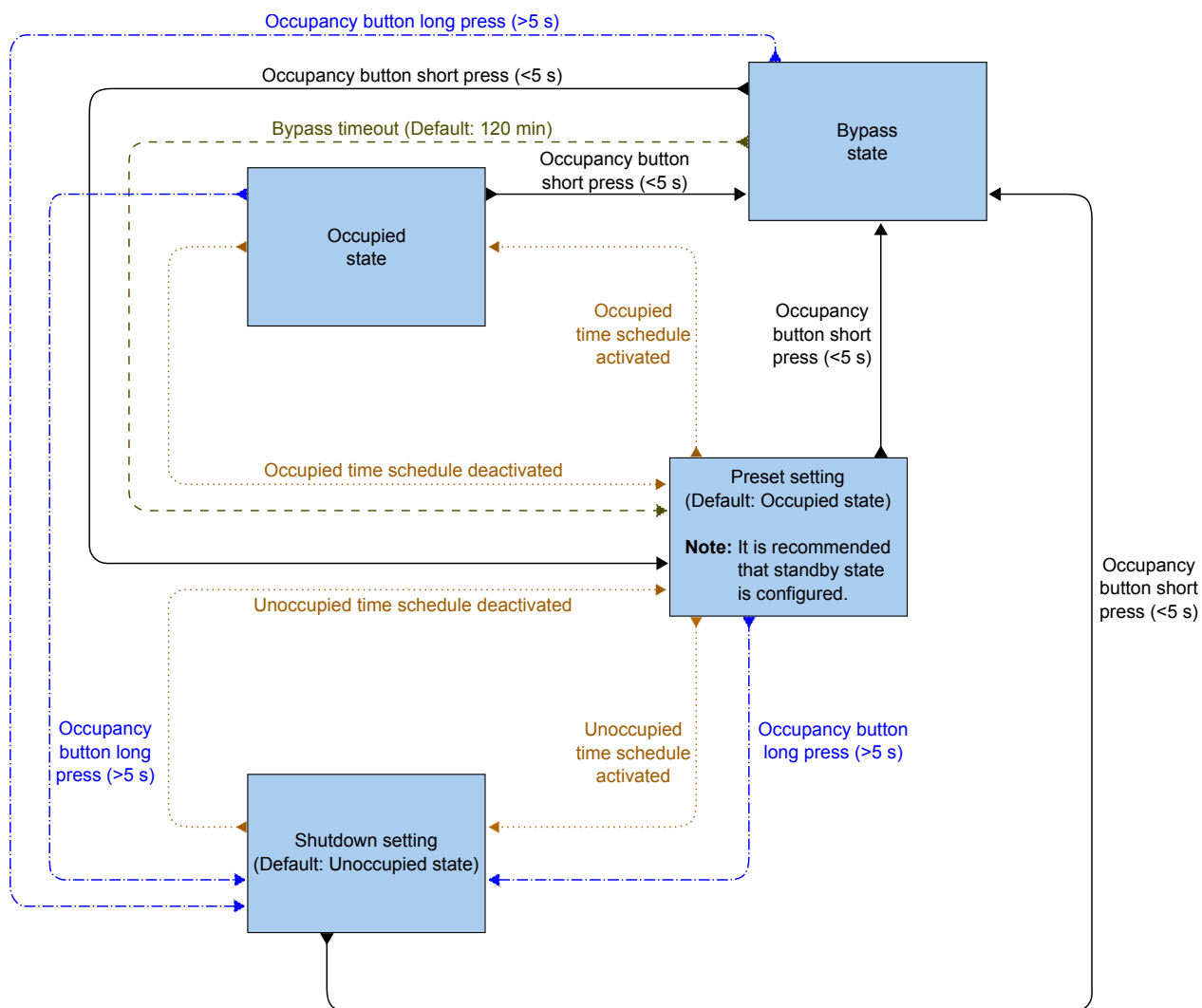
Figure 3-31 Flow chart describing controller state changes for when schedules and the occupancy (on/off) button on the room unit are used.
