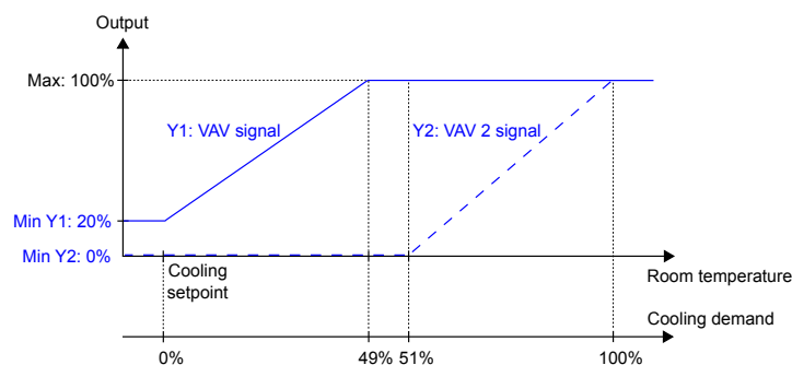
Figure 3-18 Control behaviour for the VAV + VAV controller mode when the controller regulates based on cooling demand.
