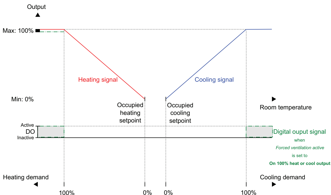
Figure 3-43 Example of forced ventilation control behaviour for the Heating + VAV controller mode when the controller is in bypass state.
