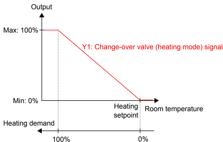
Figure 3-14 Control behaviour for the Heating/Cooling (change-over) controller mode when the controller is in heating mode.
