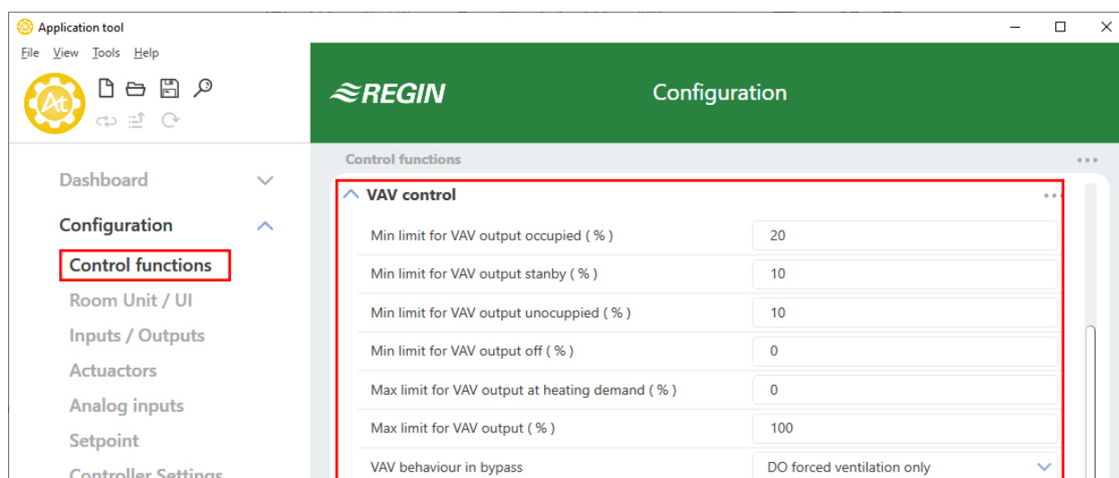
Figure 3-39 VAV control configuration settings in Application tool.
