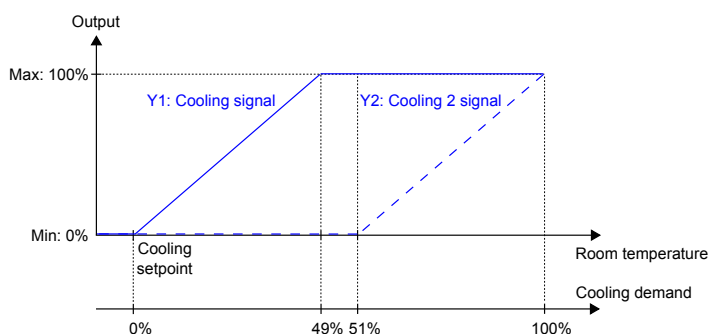
Figure 3-6 Control behaviour for the Cooling + Cooling controller mode.
