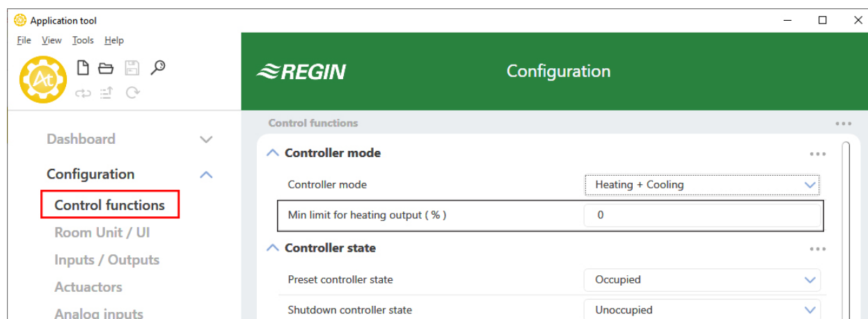
Figure 3-21 Configuration settings for minimum heating output limit in Application tool.
