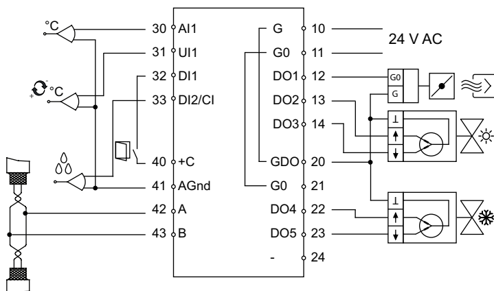
Figure 6-7 Connection diagrams for models for three-point control.
