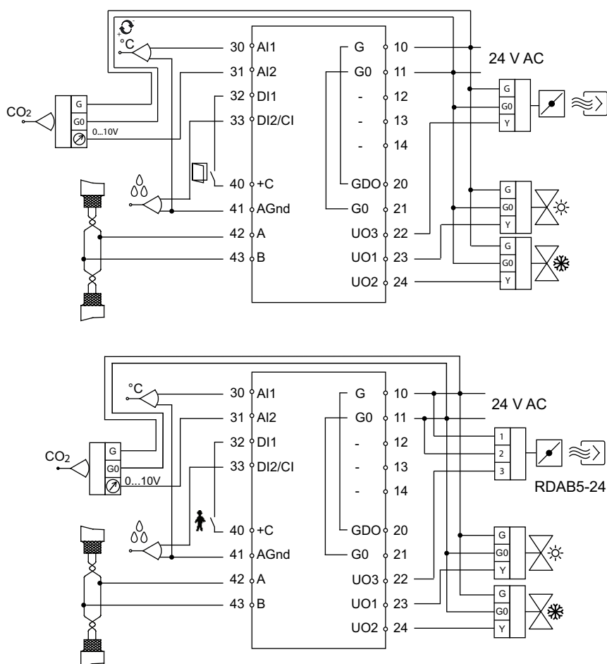
Figure 6-3 Connection diagrams for model for CO 2 control.
