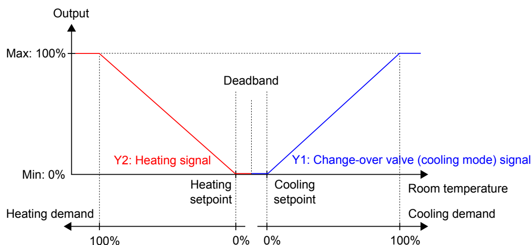
Figure 3-13 Control behaviour for the Heating + Heating/Cooling (change-over) controller mode when the controller is in Heating + Cooling mode.
