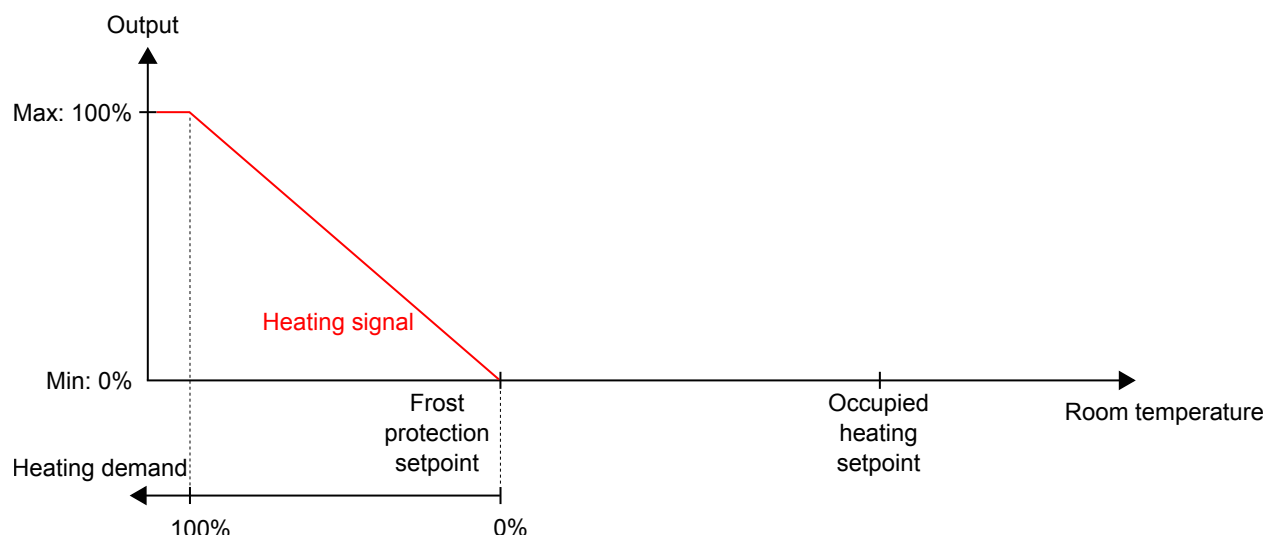
Figure 3-25 Control behaviour for the off controller state.
