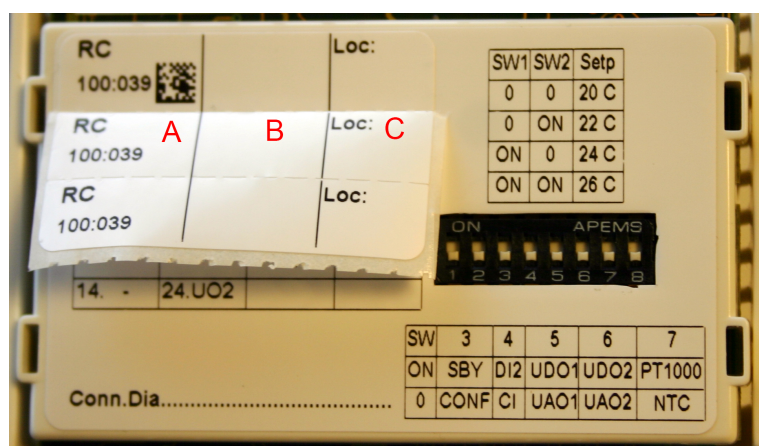
Figure 5-1 Label on the back of the controller. A: model and address. B: Field for new address or reference to connection diagram. C: Field for room number.
