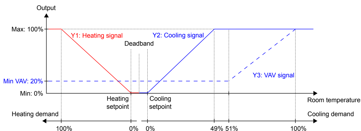
Figure 3-11 Control behaviour for the Heating + Cooling + VAV controller mode when the controller regulates based on heating and cooling demand.
