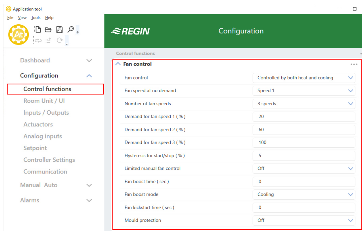
Figure 3-35 3-speed fan control configuration settings in Application tool.
