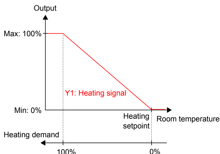
Figure 3-2 Control behaviour for the Heating controller mode.
