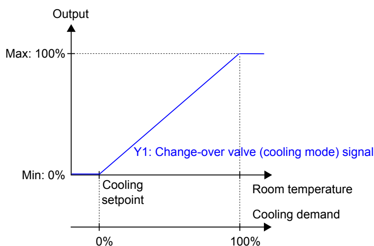
Figure 3-15 Control behaviour for the Heating/Cooling (change-over) controller mode when the controller is in cooling mode.
