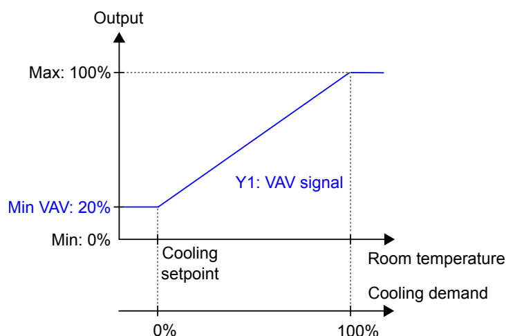
Figure 3-17 Control behaviour for the VAV controller mode when the controller regulates based on cooling demand.
