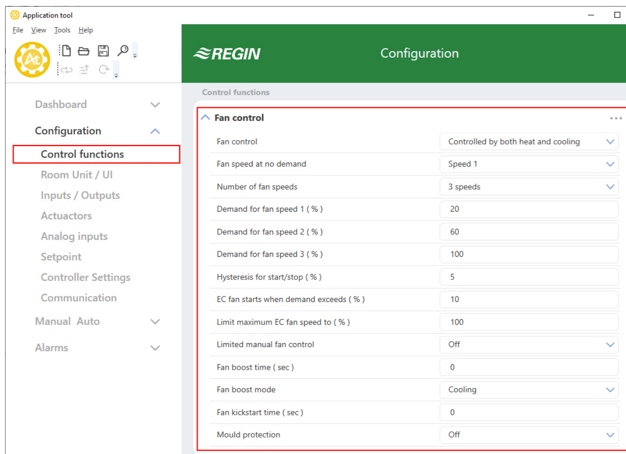
Figure 3-32 EC fan control configuration settings in Application tool.
