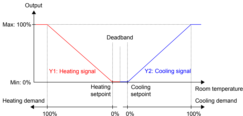
Figure 3-4 Control behaviour for the Heating + Cooling controller mode.
