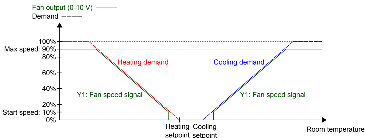
Figure 3-33 EC fan control behaviour in auto mode.
