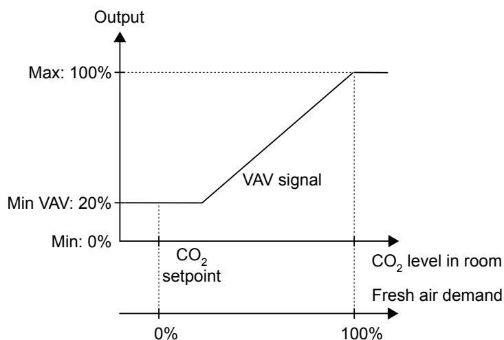
Figure 3-45 CO 2 control behaviour.
