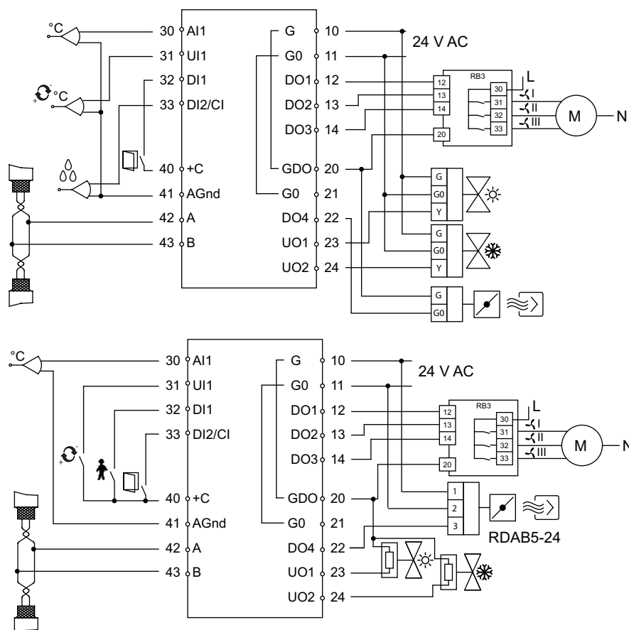
Figure 6-6 Connection diagrams for models for fan control.
