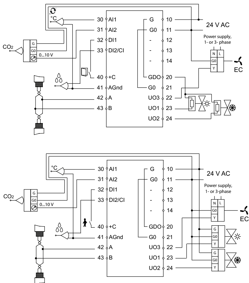
Figure 6-5 Connection diagrams for models for CO 2 control and fan control.
