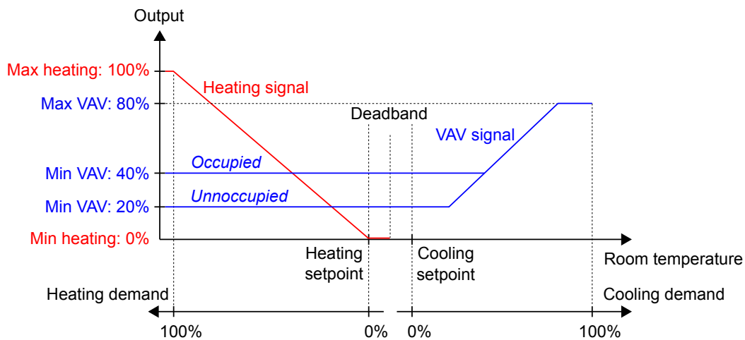
Figure 3-40 VAV control behaviour based on cooling demand when a maximum limit is set, and minimum limits for the occupied and unoccupied controller states are set.
