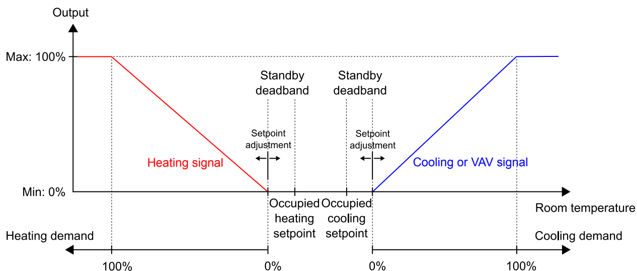
Figure 3-27 Control behaviour for the standby controller state.
