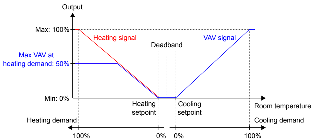
Figure 3-41 Control behaviour for the Heating + VAV controller mode when the maximum VAV output on heating demand setting is applied.
