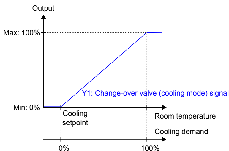
Figure 3-20 Control behaviour for the Heating/Cooling (change-over) controller mode when the controller is in cooling mode.
