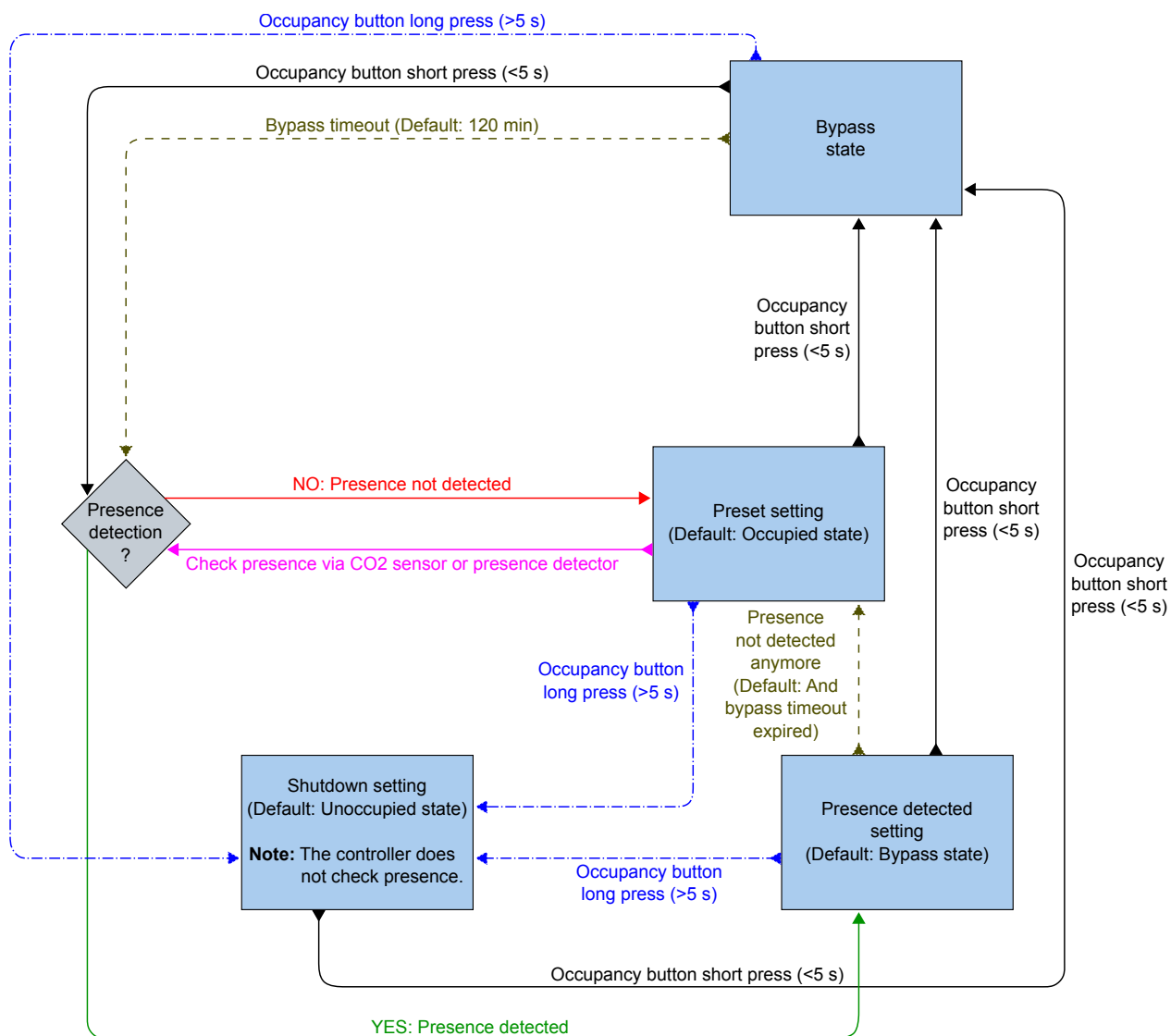
Figure 3-30 Flow chart describing controller state changes for when presence detection and the occupancy (on/off) button on the room unit are used.
