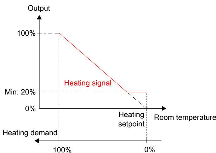
Figure 3-22 Control behaviour when maximum and minimum limits are set for the heating output.
