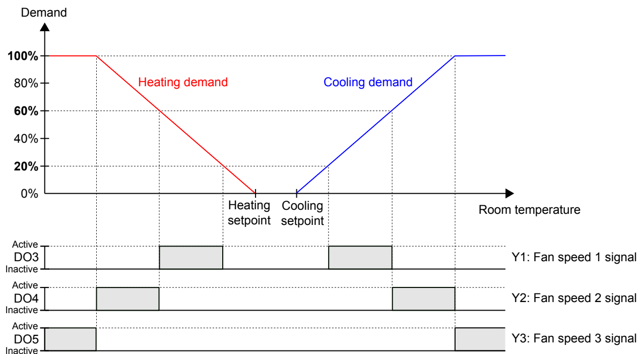
Figure 3-36 3-speed fan control behaviour in auto mode.
