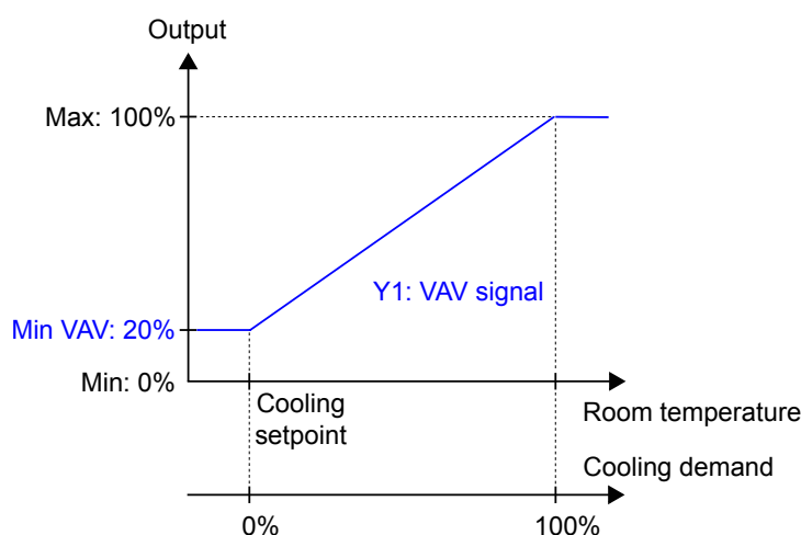
Figure 3-16 Control behaviour for the VAV controller mode when the controller regulates based on cooling demand.
