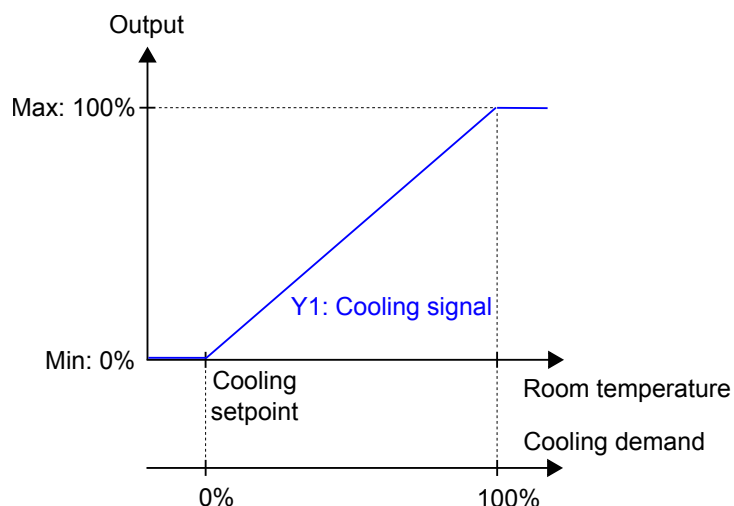
Figure 3-5 Control behaviour for the Cooling controller mode.
