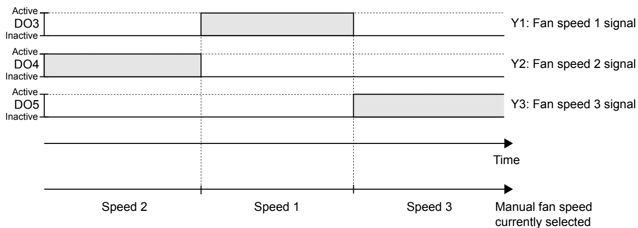
Figure 3-37 3-speed fan control behaviour in manual mode (fan speed 1, 2, or 3).
