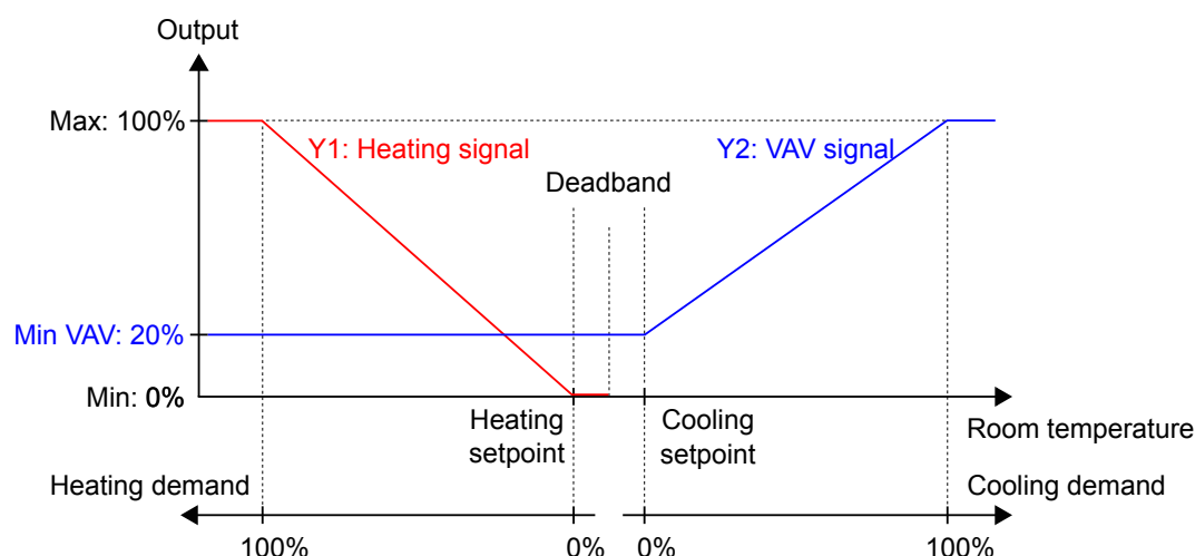
Figure 3-10 Control behaviour for the Heating + VAV controller mode when the controller regulates based on heating and cooling demand.
