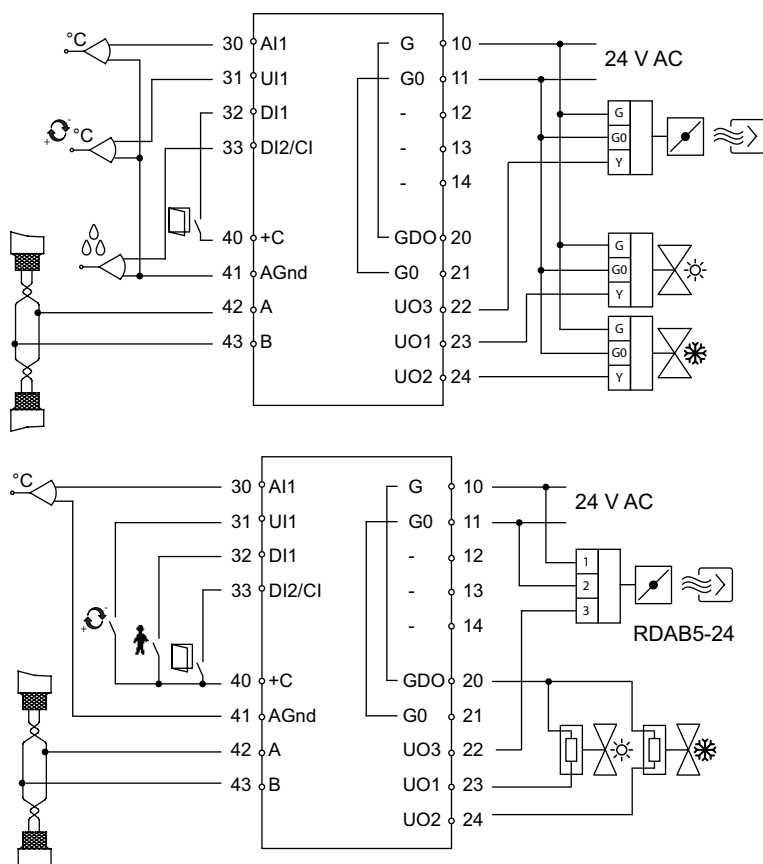
Figure 6-2 Connection diagrams for basic models with 3 universal outputs.
