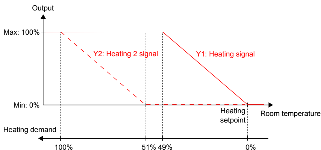
Figure 3-3 Control behaviour for the Heating + Heating controller mode.
