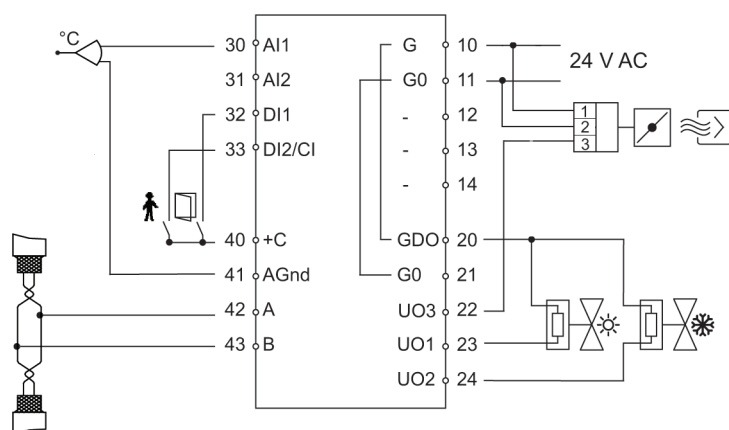
Figure 6-4 Connection diagrams for model with built-in CO 2 sensor.
