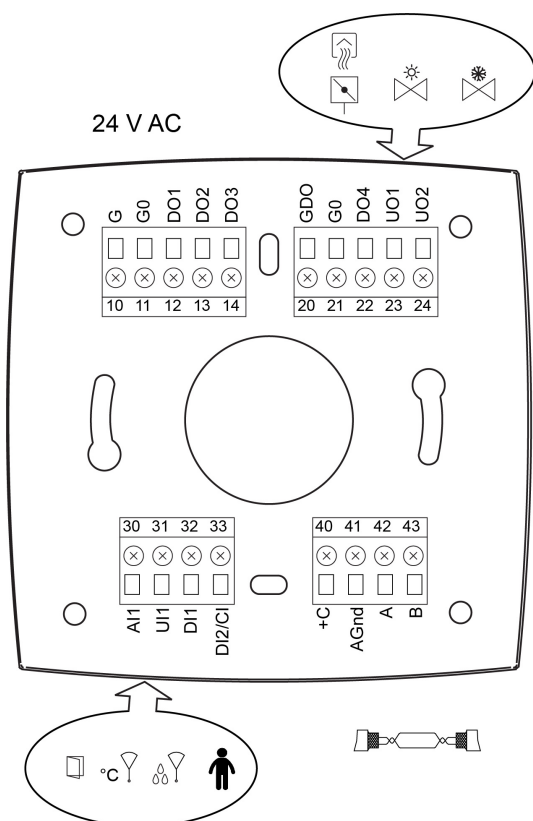
Figure 6-1 Example of bottom plate with terminals.
