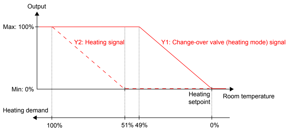
Figure 3-12 Control behaviour for the Heating + Heating/Cooling (change-over) controller mode when the controller is in Heating + Heating mode.
