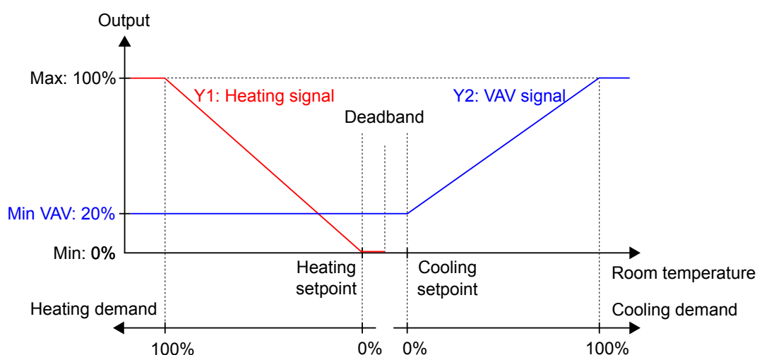
Figure 3-9 Control behaviour for the Heating + VAV controller mode when the controller regulates based on heating and cooling demand.
