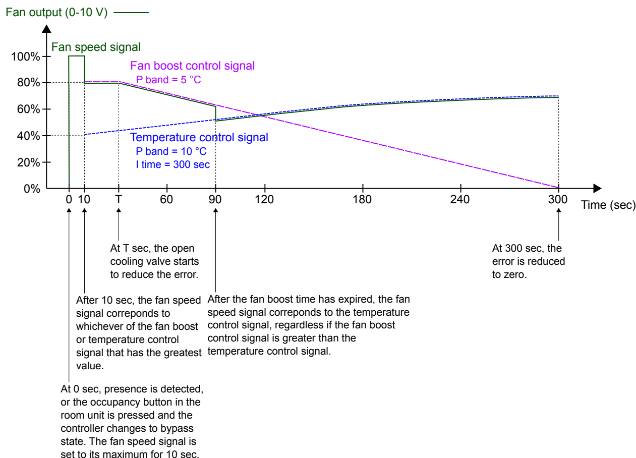
Figure 3-38 An example of fan boost control behaviour for an EC fan in auto mode, which provides a perceived cooling effect until the cooling distribution from the cooling valve establishes. The P-band for the fan boost controller has a lower value (higher gain) than the P-band for the temperature controller.
