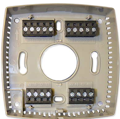
Old terminal type (1.3 mm pins).
