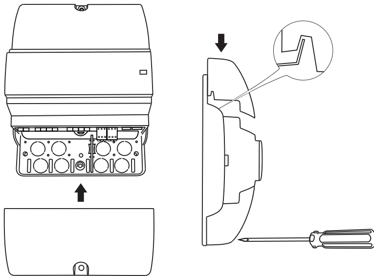
Figure 8-5 Attaching and securing the terminal protection covers.
