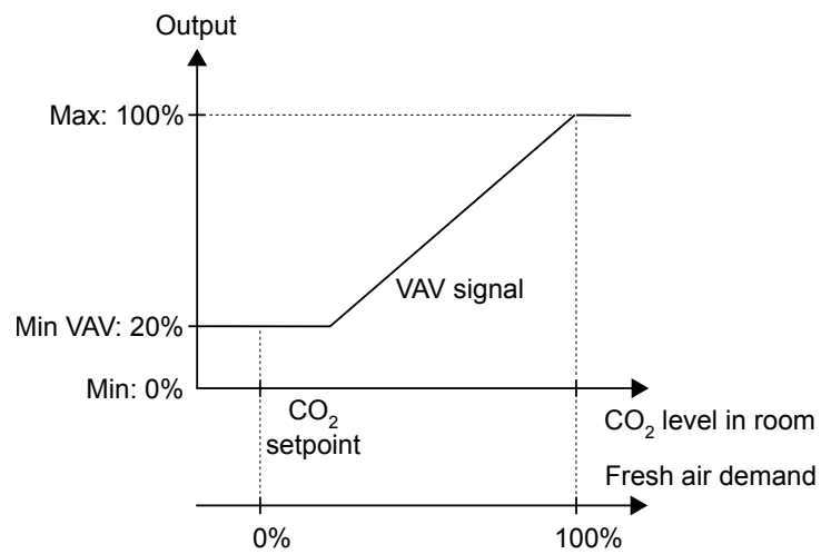
Figure 2-40 CO 2 control behaviour.
