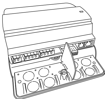
Figure 8-4 The pre-mounted partition on the baseplate.
