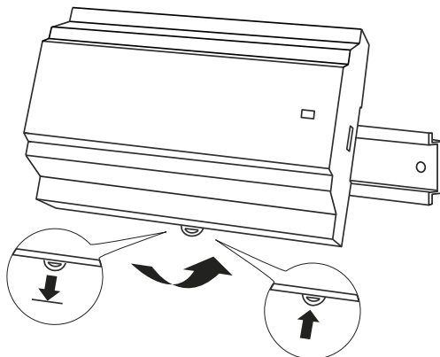
Figure 8-1 Attaching the controller to the DIN rail.
