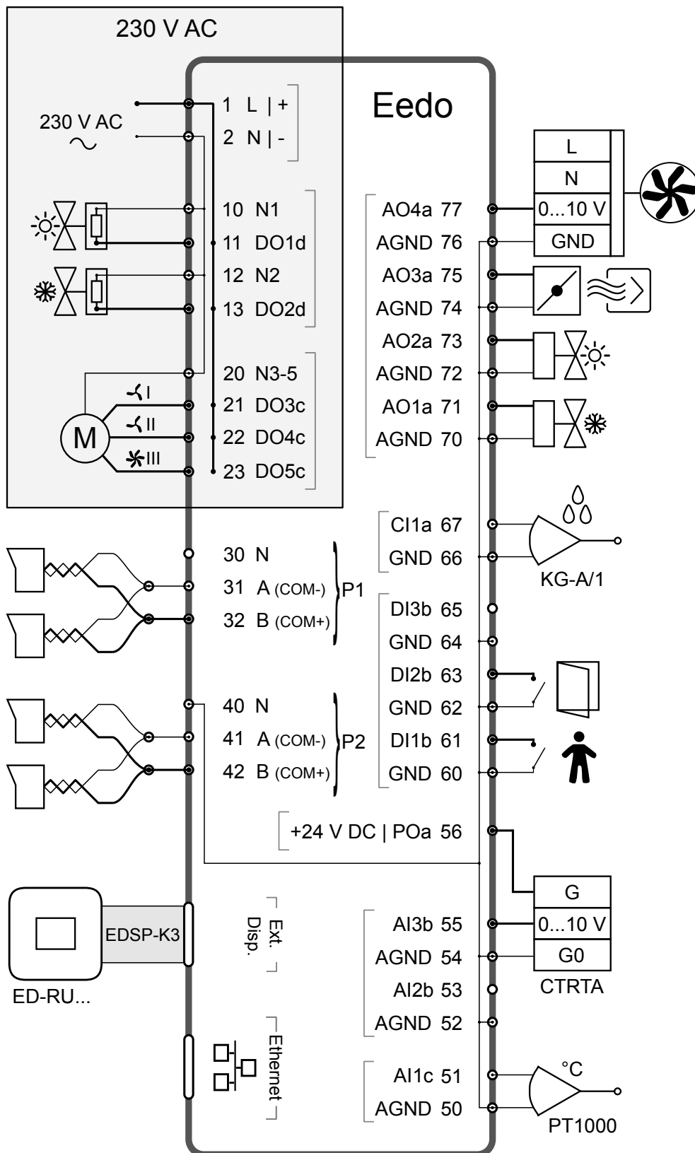
Figure 6-2 Wiring diagram exemplifying controller connections usage.
