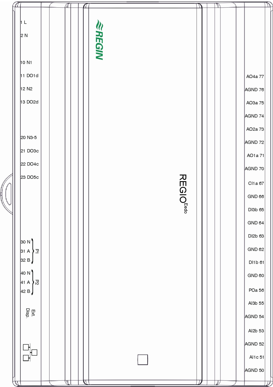
Figure 6-1 Controller connections layout.
