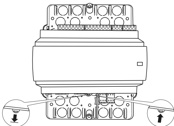
Figure 8-3 Attaching the controller to the baseplate.
