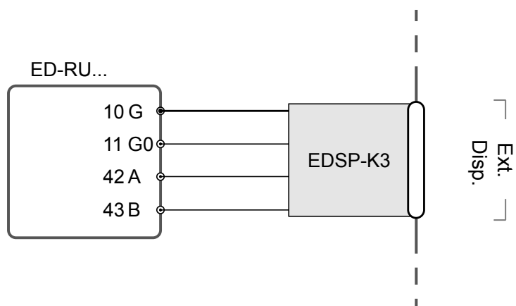
Figure 6-3 Wiring diagram for the ED-RU... room unit.
