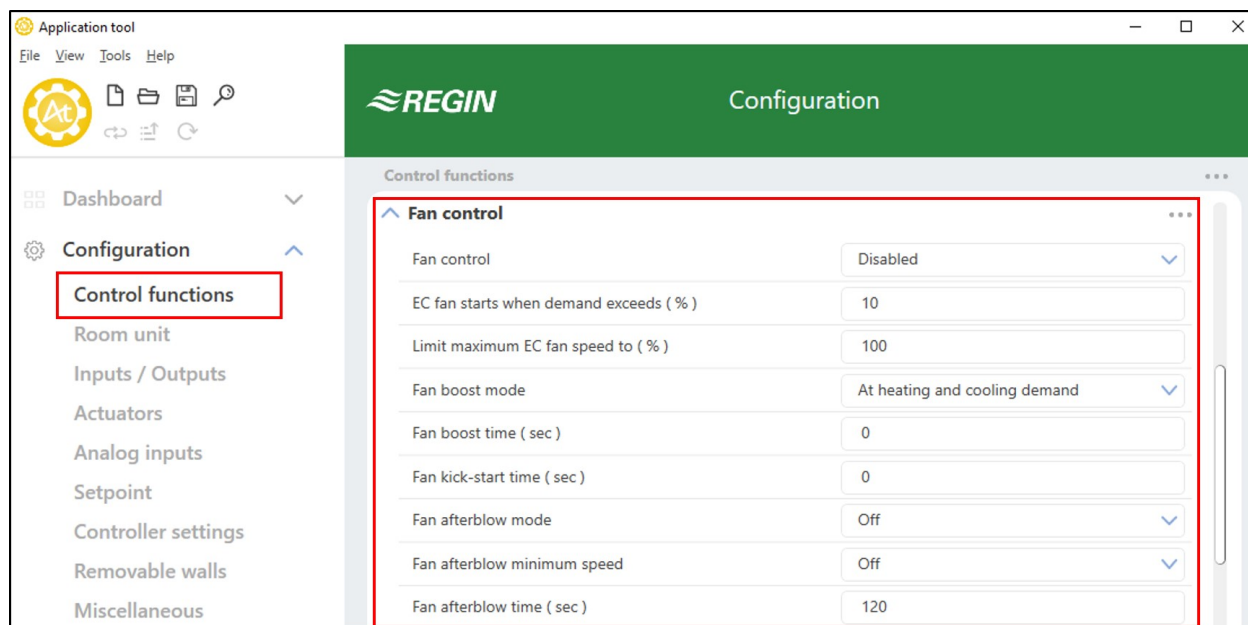
Figure 2-26 EC fan control configuration settings in Application tool.
