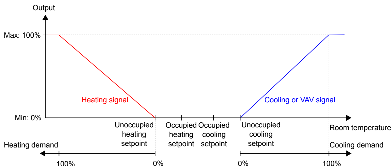
Figure 2-20 Control behaviour for the unoccupied controller state.
