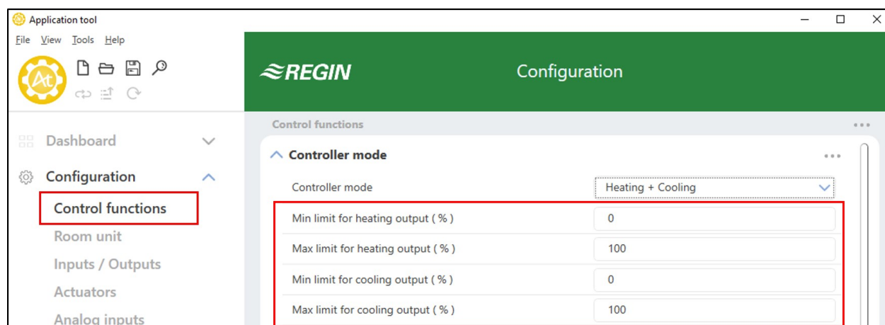
Figure 2-14 Configuration settings for maximum and minimum heating and cooling output limits in Application tool.
