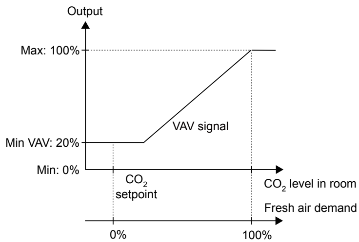
Figure 2-42 CO 2 control behaviour.
