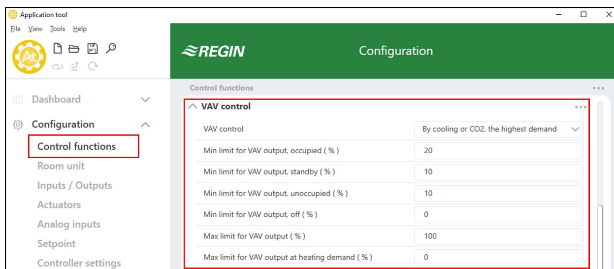
Figure 2-33 VAV control configuration settings in Application tool.
