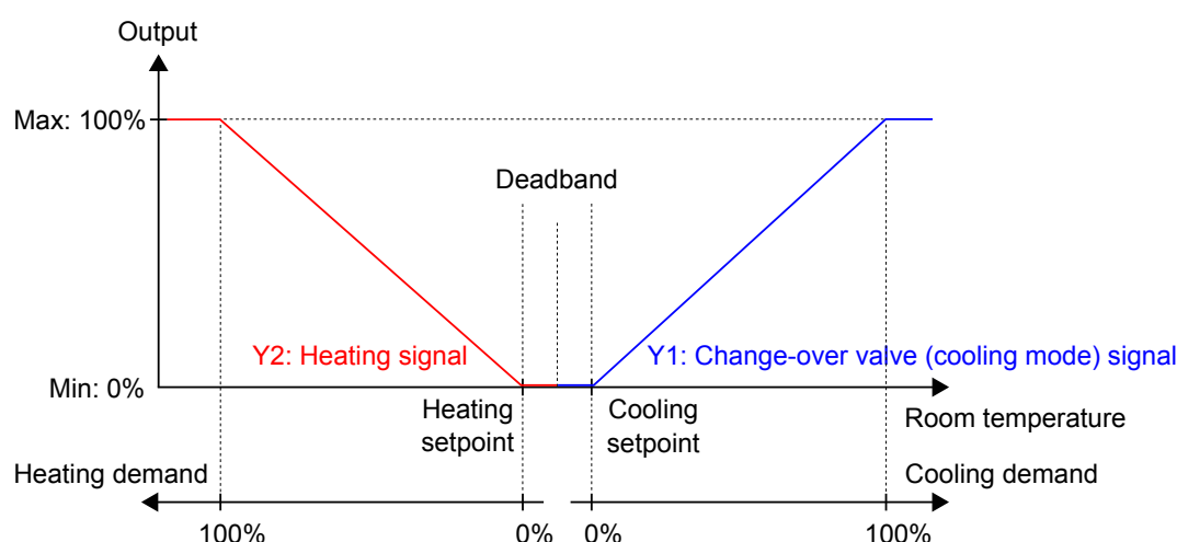
Figure 2-9 Control behaviour for the Heating + Heating/Cooling (change-over) controller mode when the controller is in Heating + Cooling mode.
