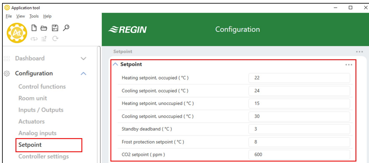
Figure 5-1 Setpoint and deadband configuration settings in Application tool.
