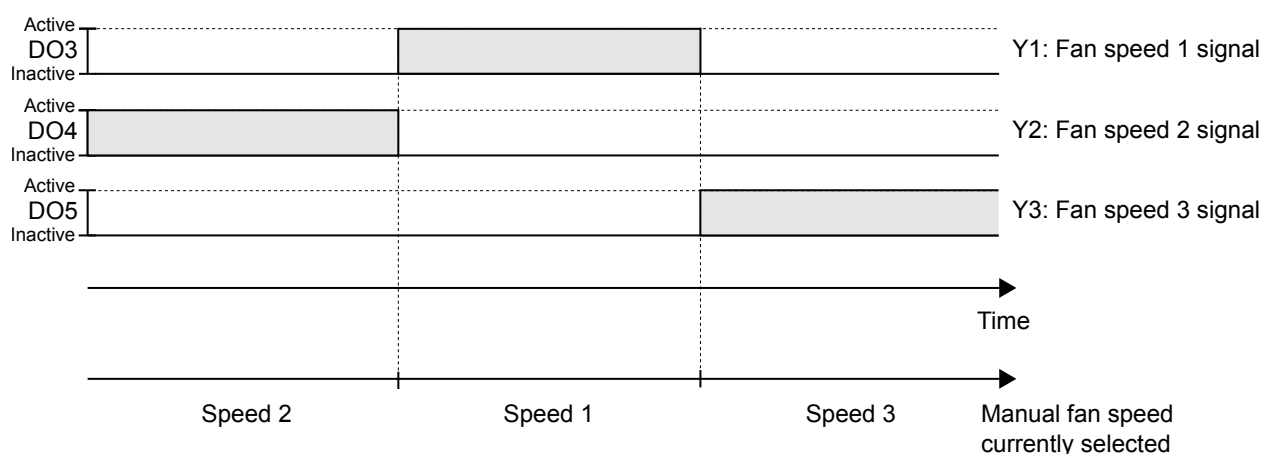
Figure 2-31 3-speed fan control behaviour in manual mode (fan speed 1, 2, or 3).
