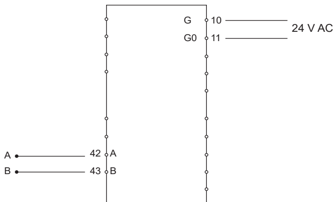
Figur 1 Inkoppling
