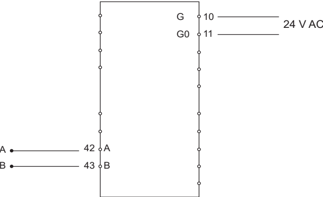
Figur 1 Inkoppling
