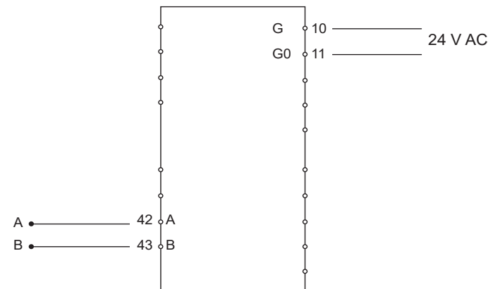
Figur 1 Inkoppling
